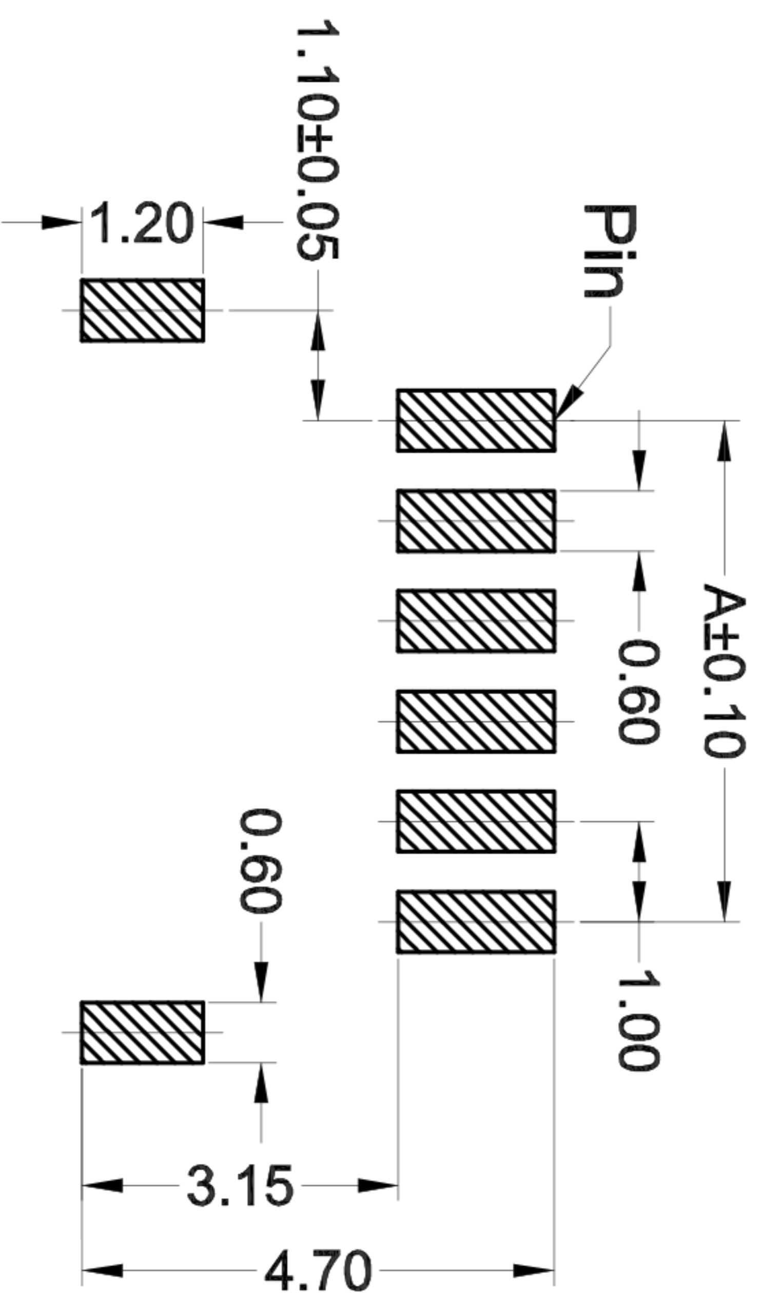
Recommended PCB hole Layout Top view (Tolerance±0.10)
