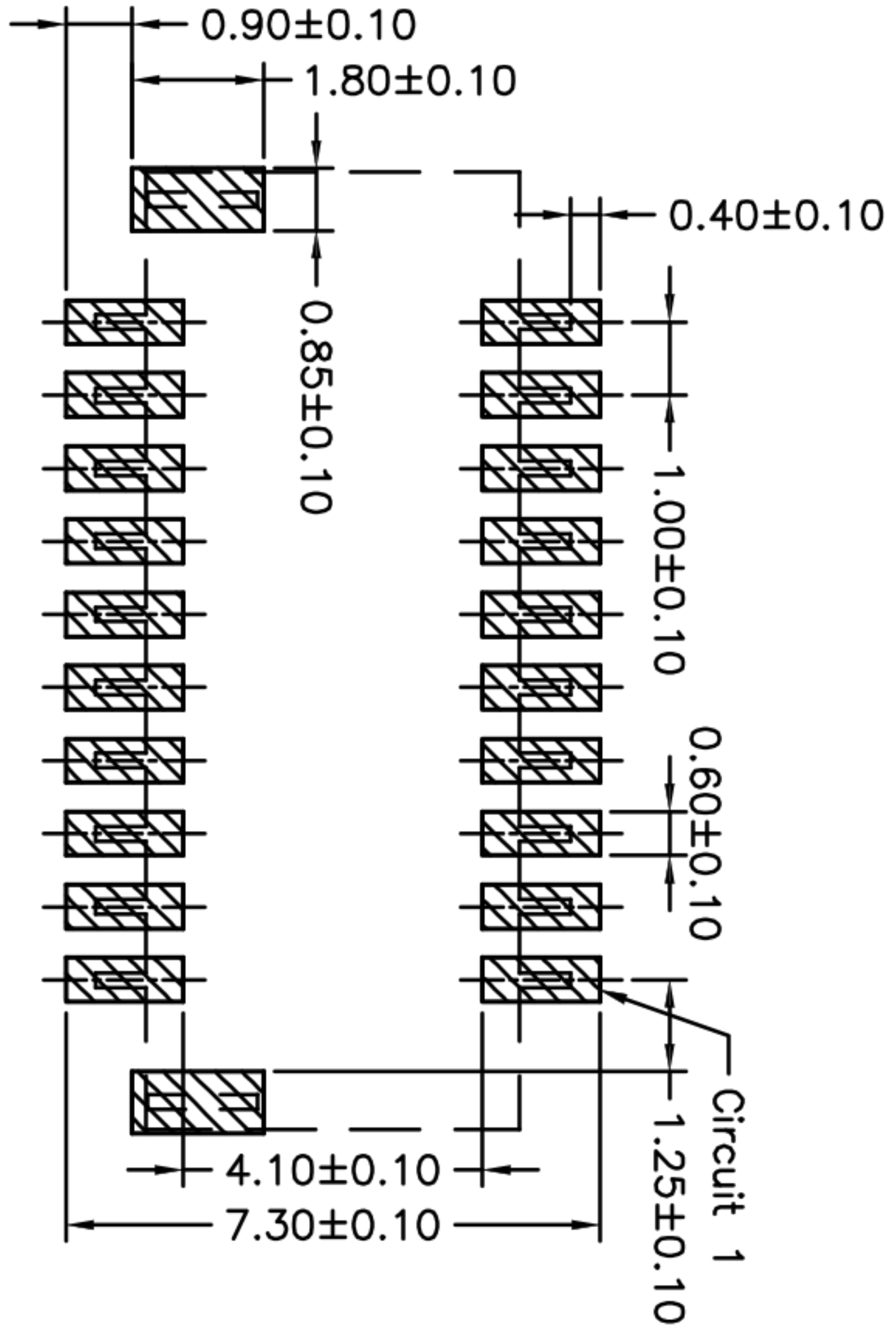
PCB LAYOUT
