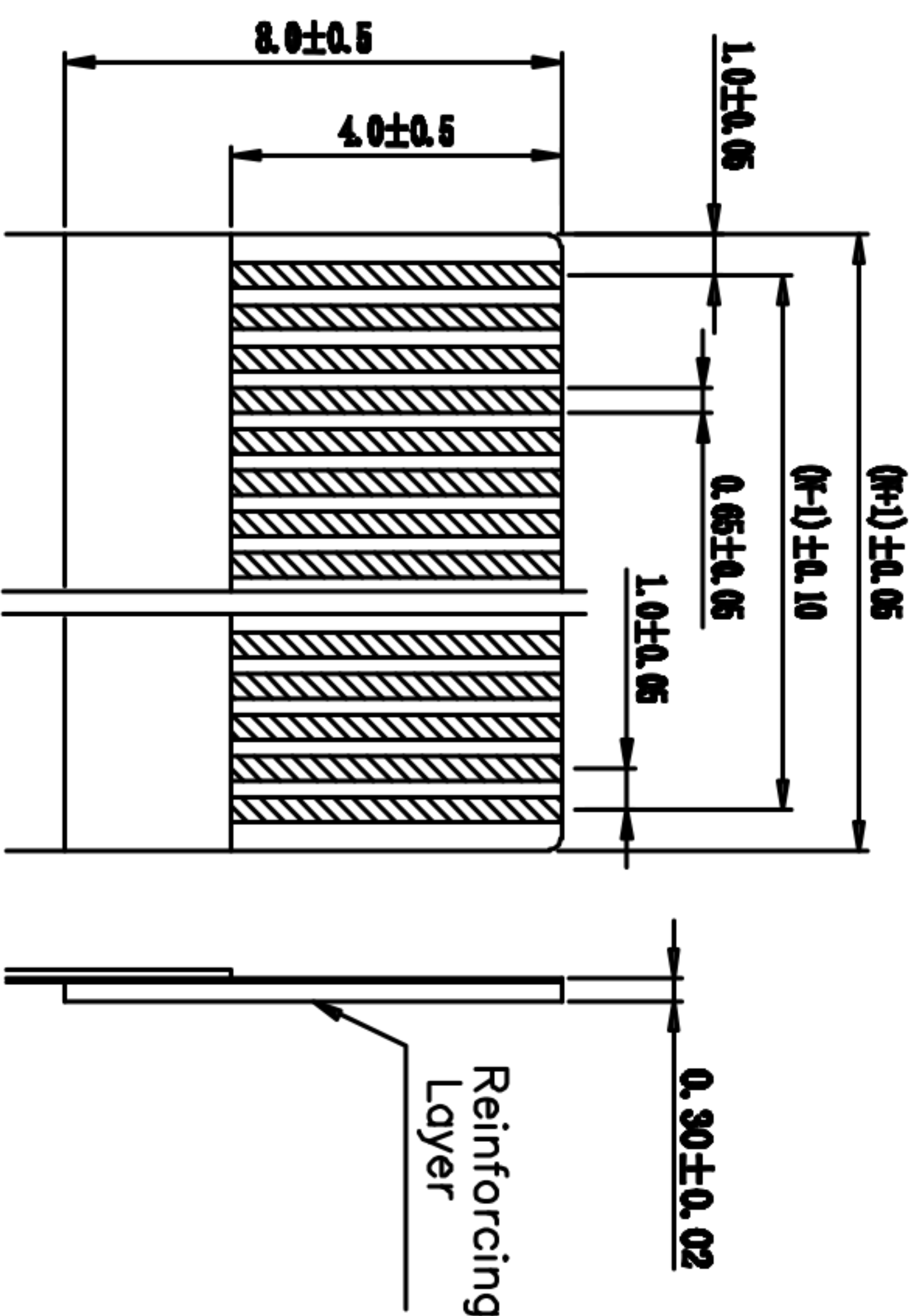
RECOMMENDED FFC/FPC DIM.
