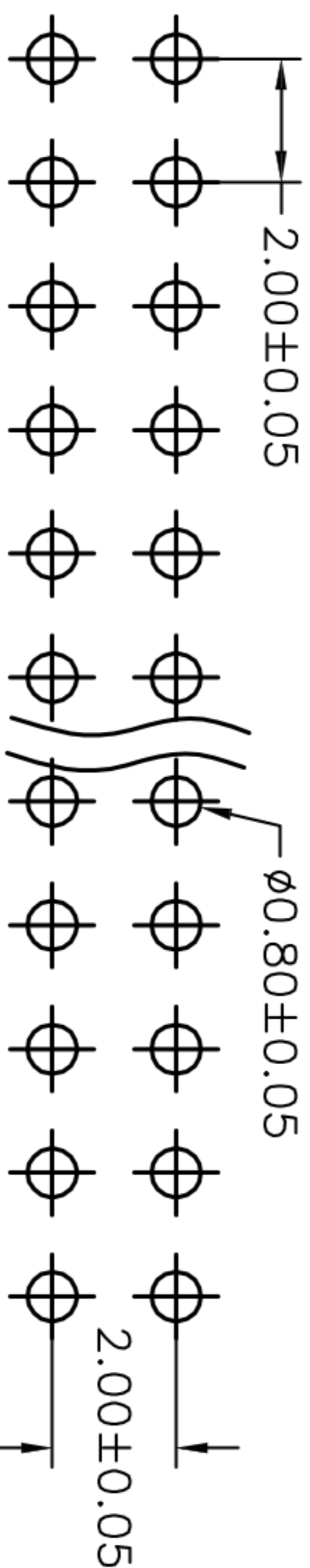
Recommended PCB Layout
